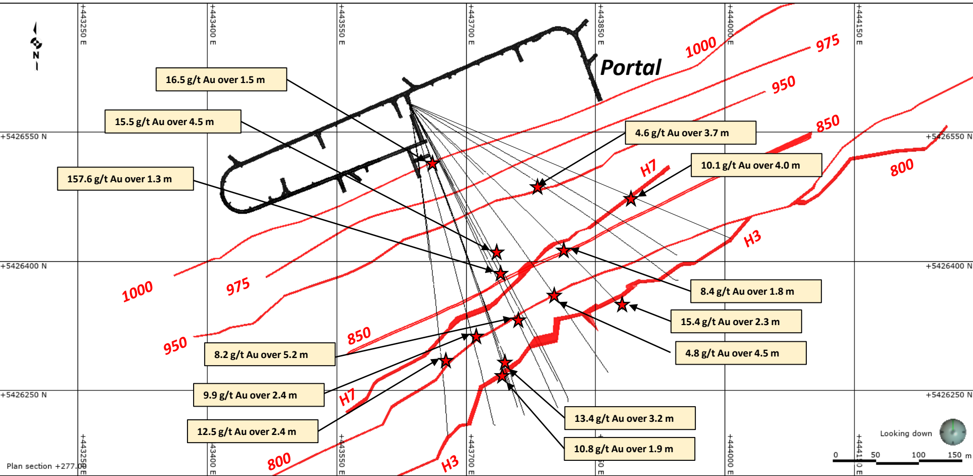
➤ Plan view – Level 100
